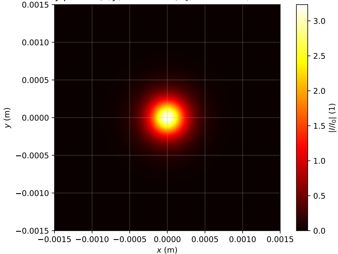
Intensity profile I(x, y, z = 3.821m)/I_0 , Pin=1.0Pcr, artificial time
